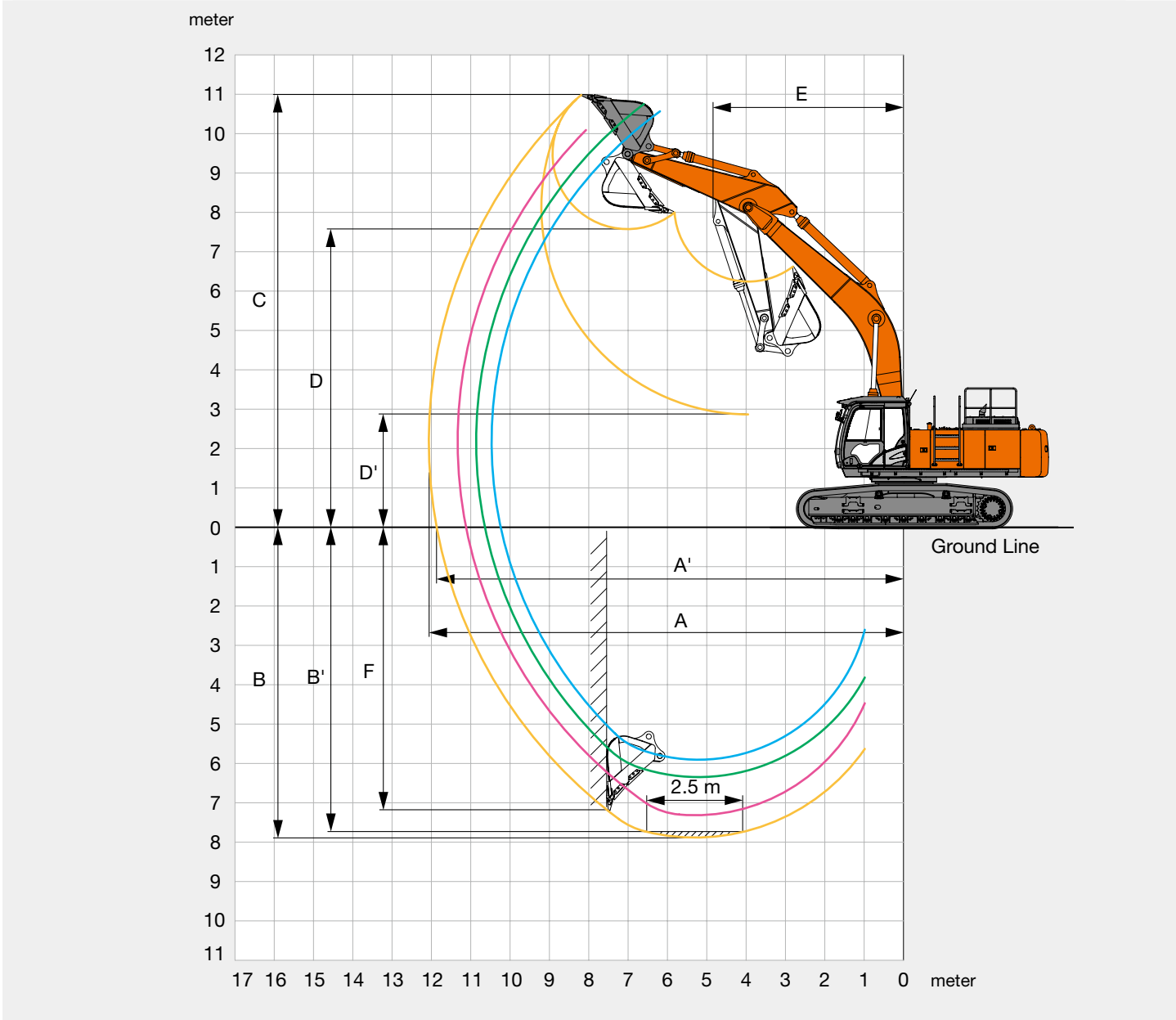
ZX470H-5G / ZX470LCH-5G
